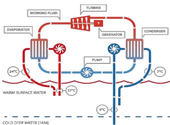
Figure 2 - Ocean Thermal Energy Conversion Cycle
