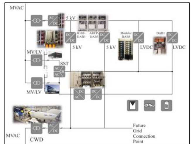
Demo2: RWTH Aachen MV/LVDC Campus grid
